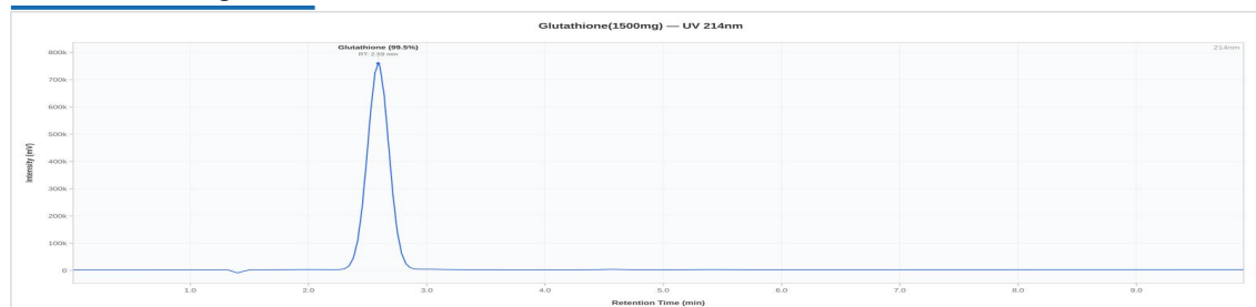
Glutathione 1500mg - 032026: UV Chromatogram
